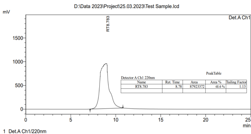
Figure 3: The HPLC Chromatogram of Test Sample (enzymatic treated) assayed in this study
