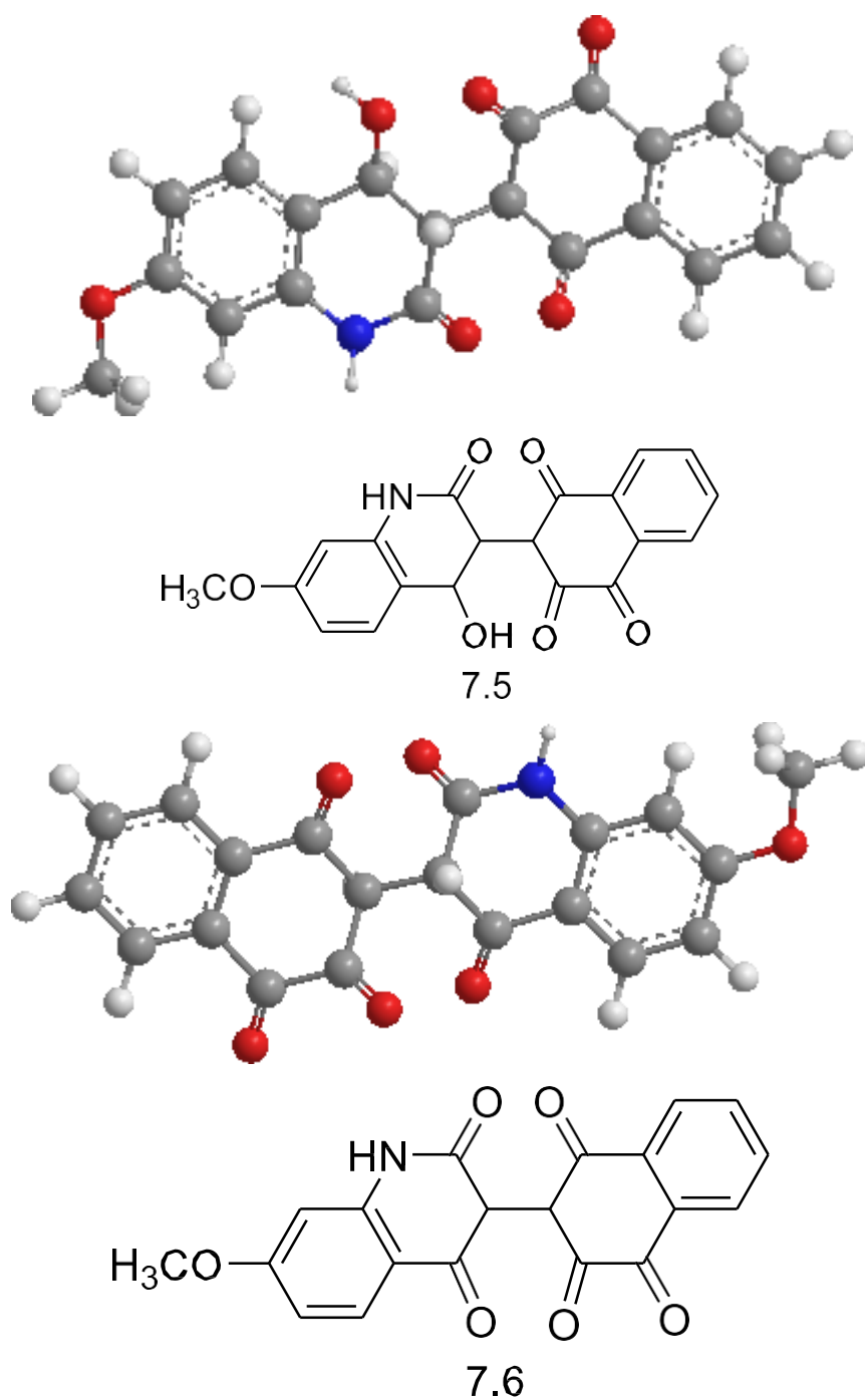
Figure 7 Optimum geometry calculation of compound 7.
