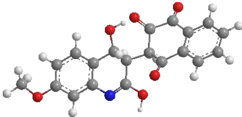
Figure 7 Optimum geometry calculation of compound 7.
