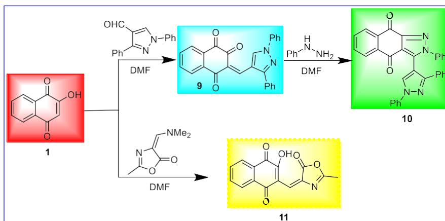
Scheme 2 Synthesis of some binary compounds 9–11.
