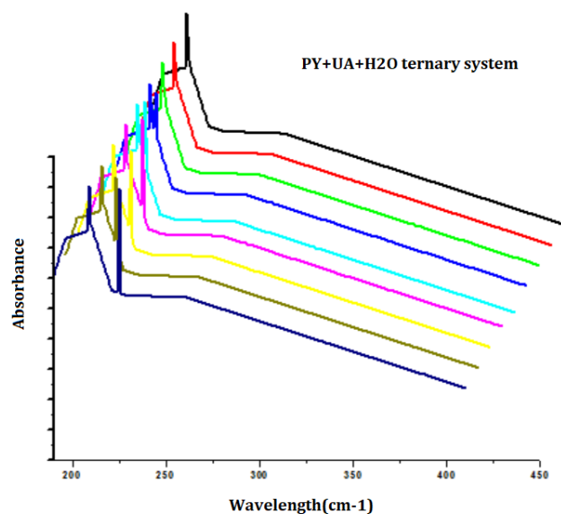
Figure 6b. UV spectra for pyridoxal phosphate in the presence of aqueous uric acid at room temperature
