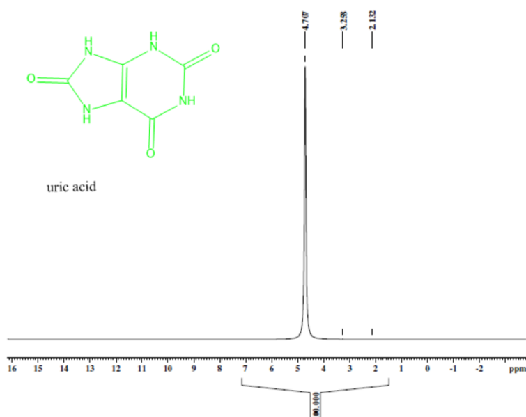
Figure 7b. NMR spectra for UA in D 2 O
