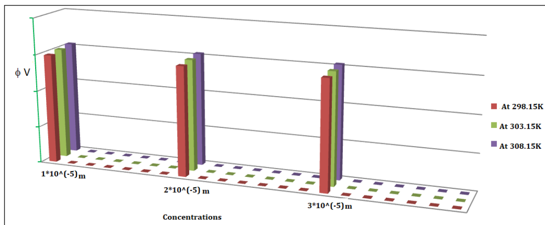
Figure 1b. Plot of the variation \phi_V of solutions as a function of molality ( m ) for UA-H 2 O solutions of pyridoxine at T = 298.15 \text{ K}, 303.15 \text{ K}, 308.15 \text{ K} .
