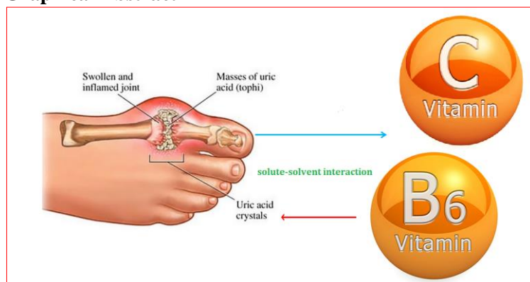
Scheme 2. Possible scheme for solute solvent interaction for PY-UA
