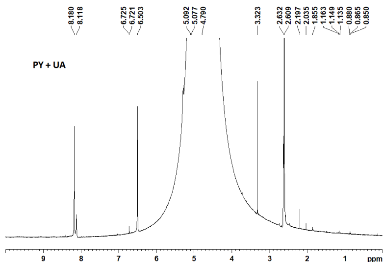
Figure 7c. NMR spectra for the mixture of PY + UA in D 2 O
