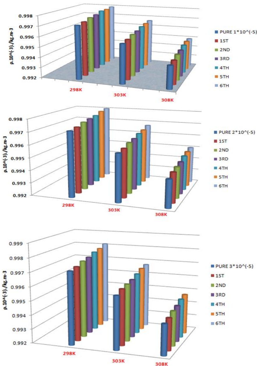
Figure 1a. Plot of the variation of density ( \rho ) of solutions as a function of molality ( m ) for UA-H 2 O solutions of pyridoxine at T = 298.15 \text{ K}, 303.15 \text{ K}, 308.15 \text{ K} .
