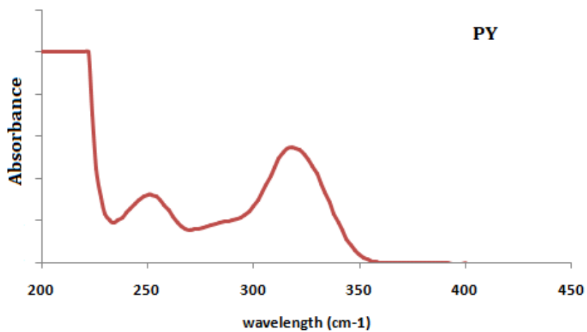
Figure 6a. UV spectra for pure pyridoxal phosphate
