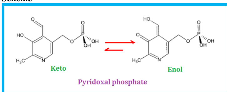
Scheme 1. Representation of the exchange of hydrogen atom in PY
