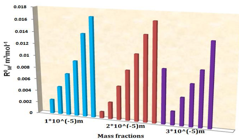
Figure 4. Plot of limiting molar refraction ( R_M^0 ) vs. mass fraction for 1 \times 10^{-5} m (sky blue), 2 \times 10^{-5} m (brown), 3 \times 10^{-5} m (purple) of PY in aqueous UA.
