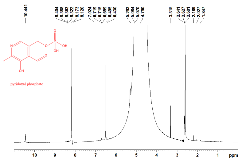
Figure 7a. NMR spectra for PY in D 2 O
