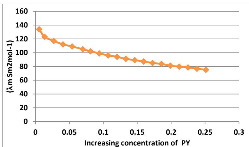
Figure 3: Plot of Molar conductance ( \Lambda_m ) against concentration in aqueous PY in mass fraction of 2 \times 10^{-5} m of the solution
