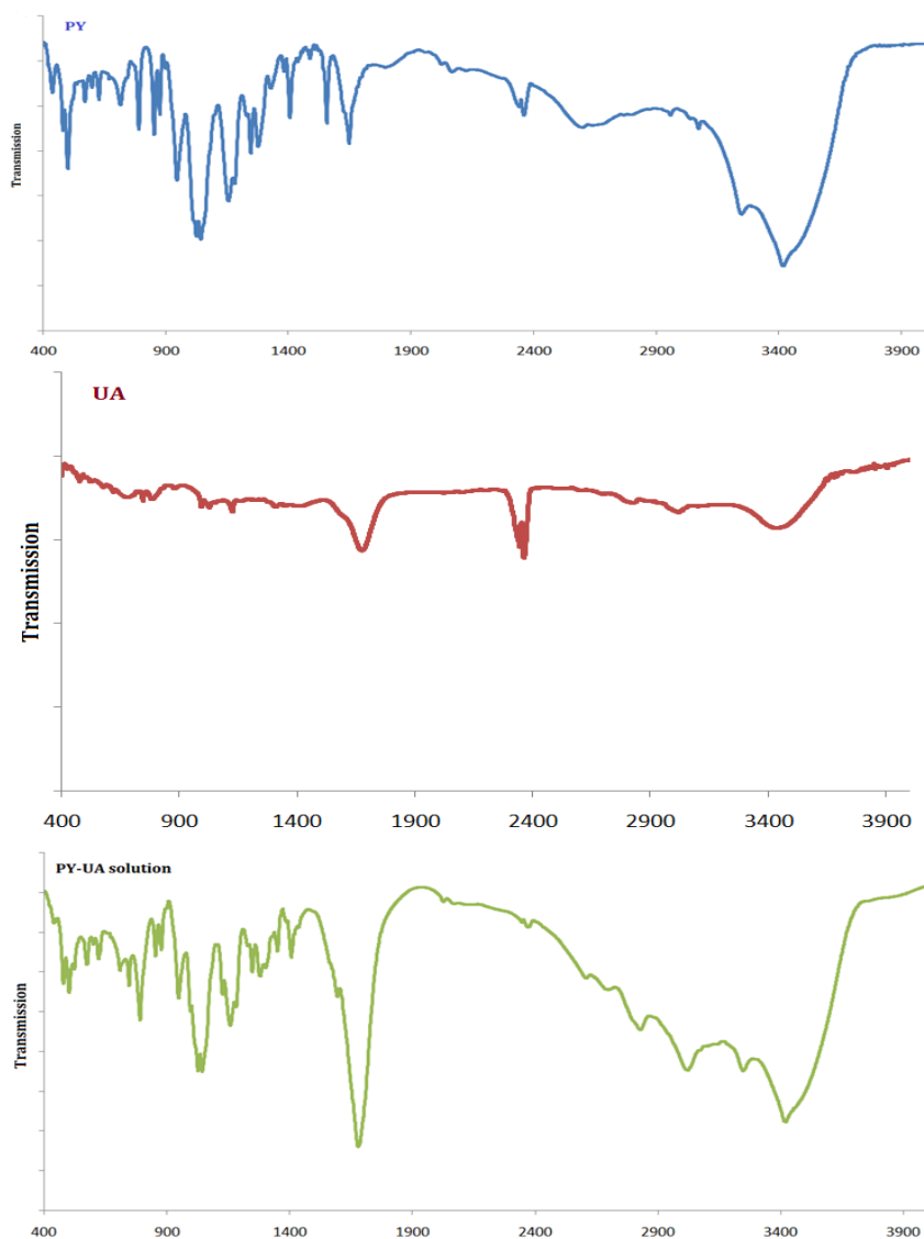
Figure 5. FTIR Spectra of pure pyridoxine phosphate (PY), uric acid (UA) and mixture of PY-UA aqueous solution
