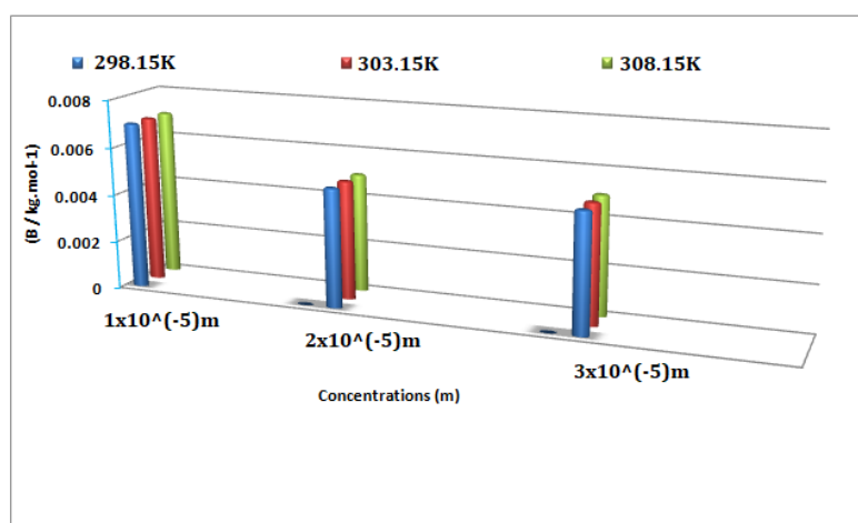
Figure 2b. Plots of viscosity B-coefficients for pyridoxine in different mole fractions in UA solutions at T = (298.15-308.15) K.
