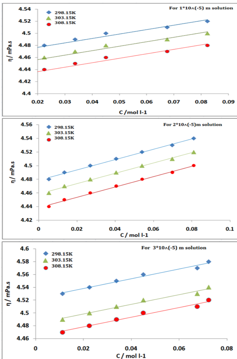
Figure 2a. Viscosities, \eta of PY in various mole fractions of UA aqueous solutions at T = 298.15 K, 303.15 K, 308.15 K
