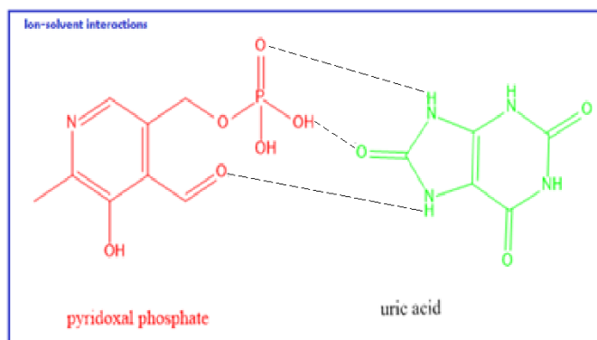
Scheme 2. Possible scheme for solute solvent interaction for PY-UA
