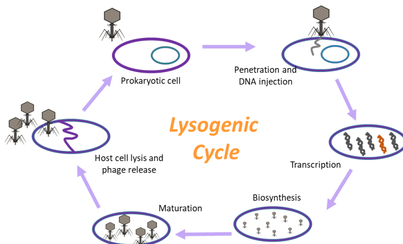
Fig. 6 Lysogenic cycle of bacteriophage.
