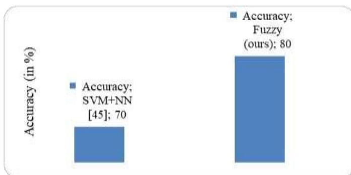
Figure 9. Accuracy Comparison
