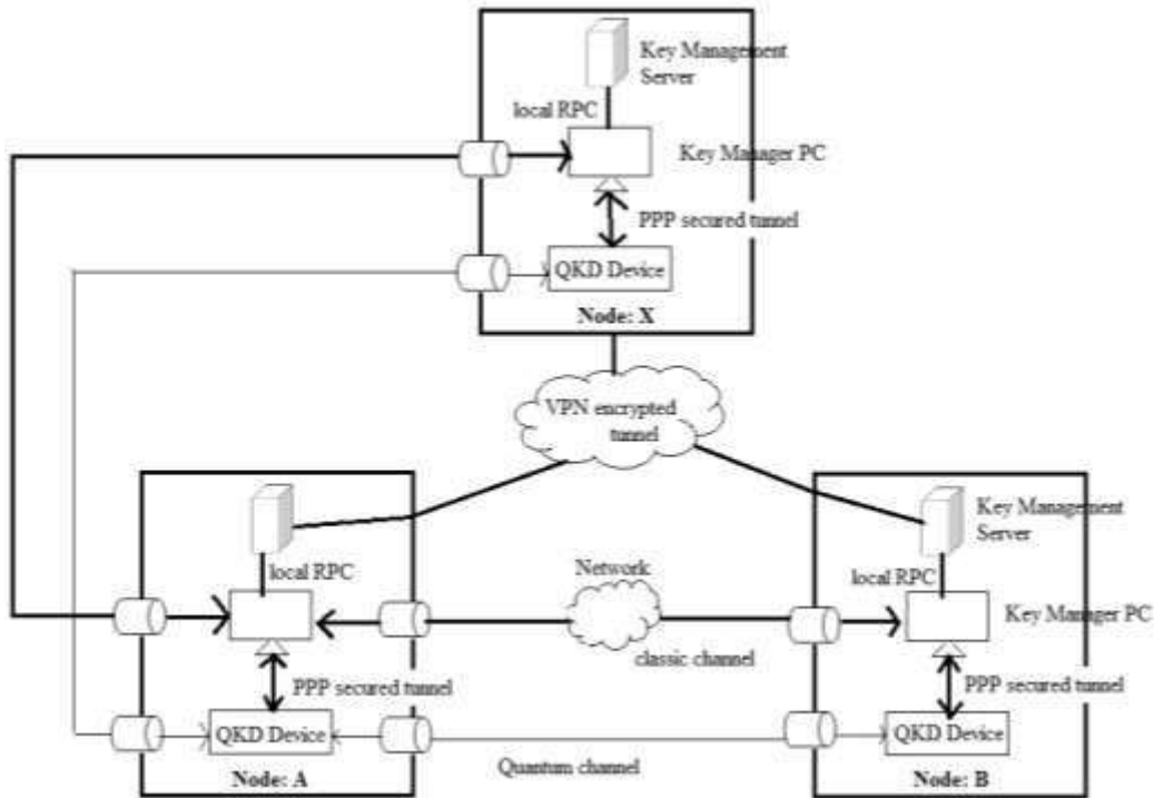
Figure 1.2 – Network infrastructure with quantum cryptography among different nodes
